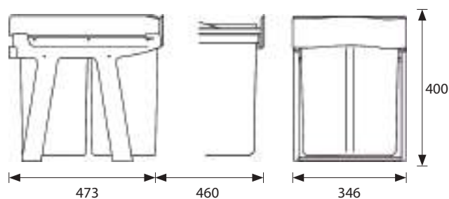
BASE 400 mm
