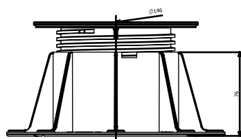
GB-K-A3 (82 -135mm)
